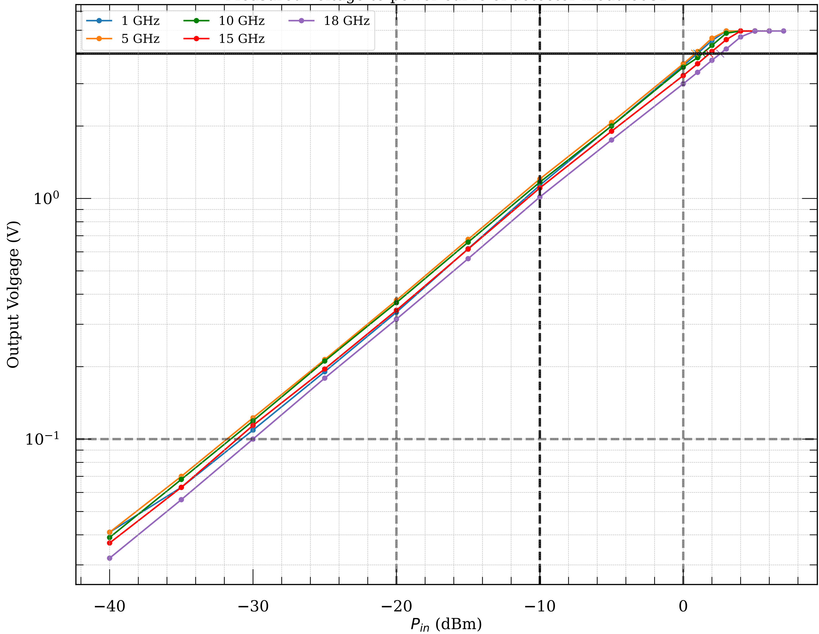
Measured voltage-to-power curve of detector module081
